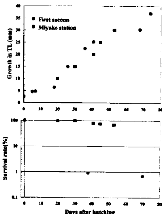
Figure 3. Comparison of growth and survival between the first success and the recent results at Miyako station of the Japan Sea-Farming Association corresponding to the development of technology.
