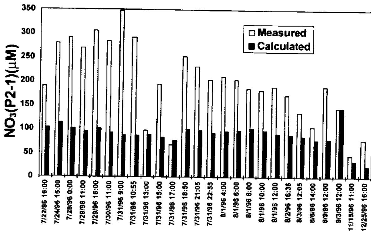
Figure 9. The variation of nitrate concentration.
