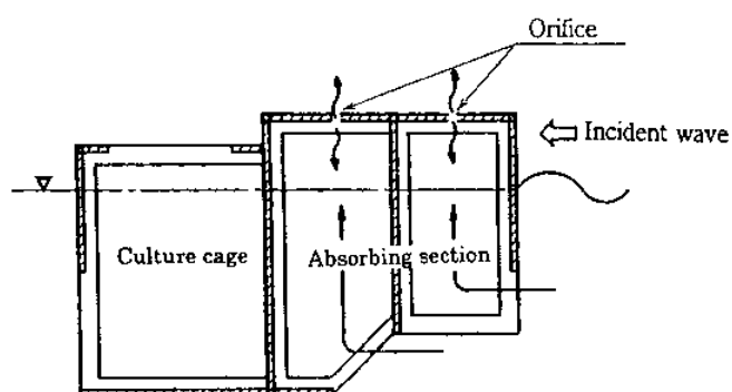
Figure 8. Cross section of the floating breakwater attached with culture cages.
