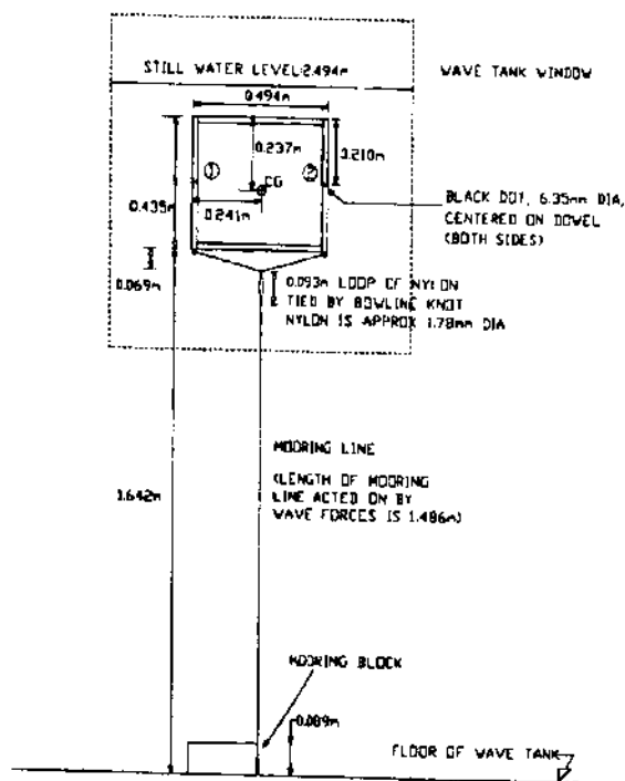
Figure 4. Experimental setup opposite upper window.
