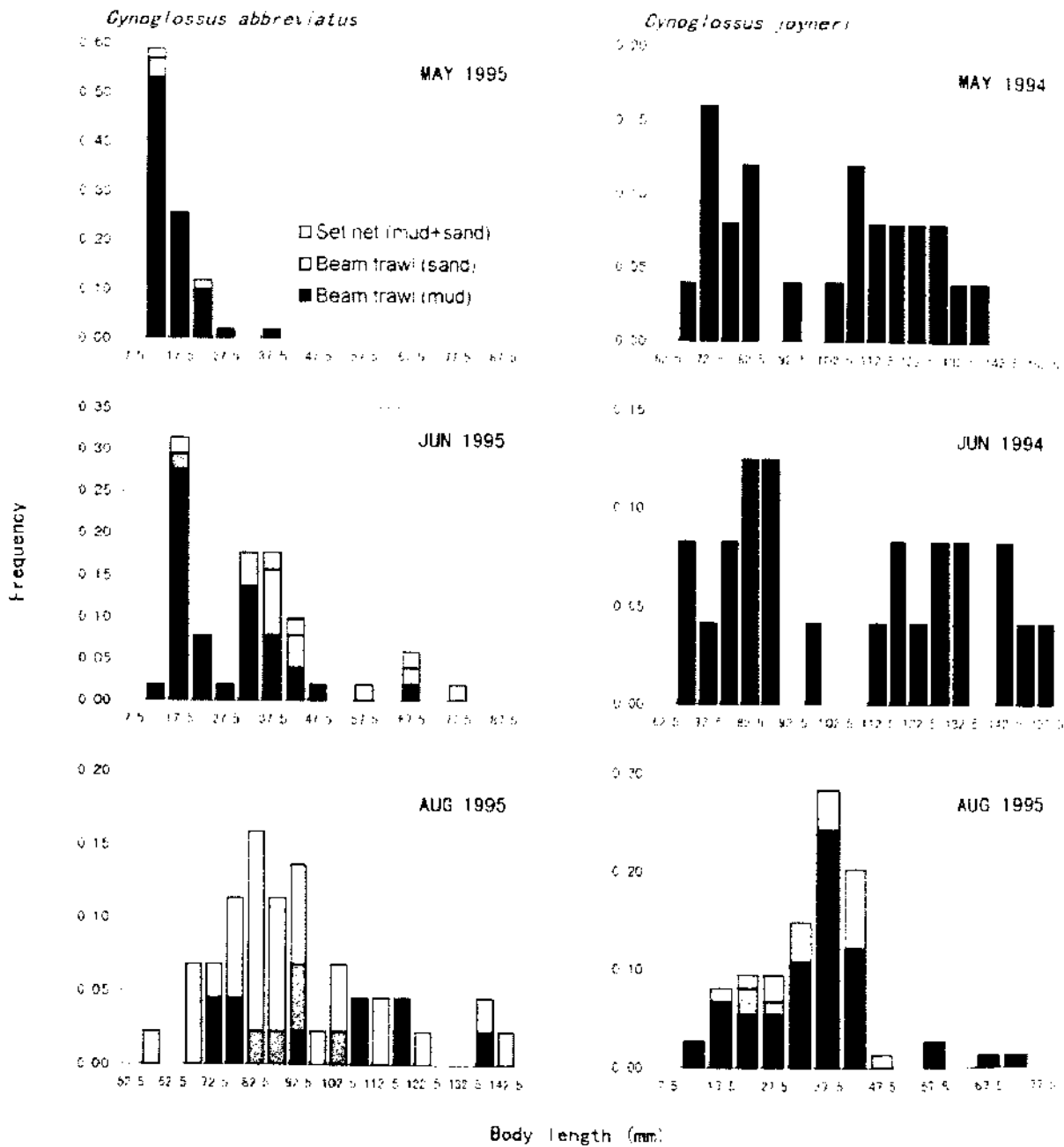
Figure 6. Body length composition of 0-group tonguefish caught by beam trawl net and set net in daytime in the sand-covered area and the muddy control area.
