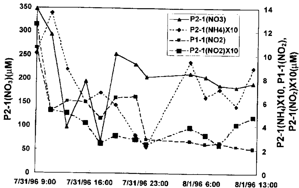
Figure 8. Time variation of nitrate, nitrite and ammonium.
