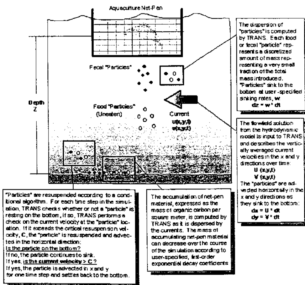
Figure 7. Summary illustration for the TRANS aquaculture net-pen waste transport simulator algorithm developed at the University of Maine.
