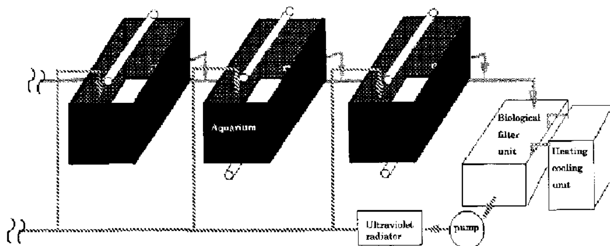
Figure 1. Experimental setup.
