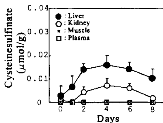
Figure 4. Changes in cysteinesulfinate contents in several tissues of rainbow trout during feeding on cystine-supplemented diet (Yokoyama and Nakazoe 1998). Results are expressed as the mean \pm standard deviation of five individuals.
