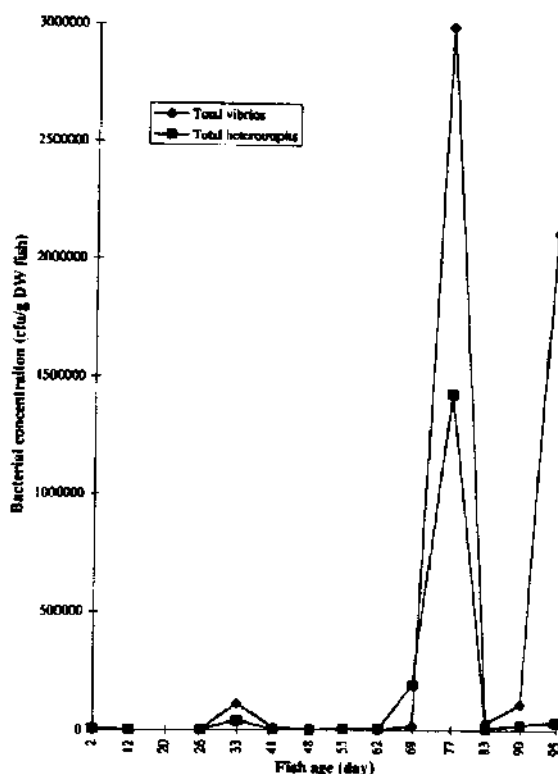
Figure 3. Bacterial concentrations in "healthy" fish. cfu = colony forming units; DW = dry weight.
