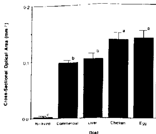
Figure 1. Mean cross-sectional area of the bolus in larval zebrafish fed spray-dried microparticulate diets over 1.5 h. Data are means \pm standard error ( n=3 ). Treatments with different subscripts are significantly different ( p<0.05 , Fisher PLSD method).
