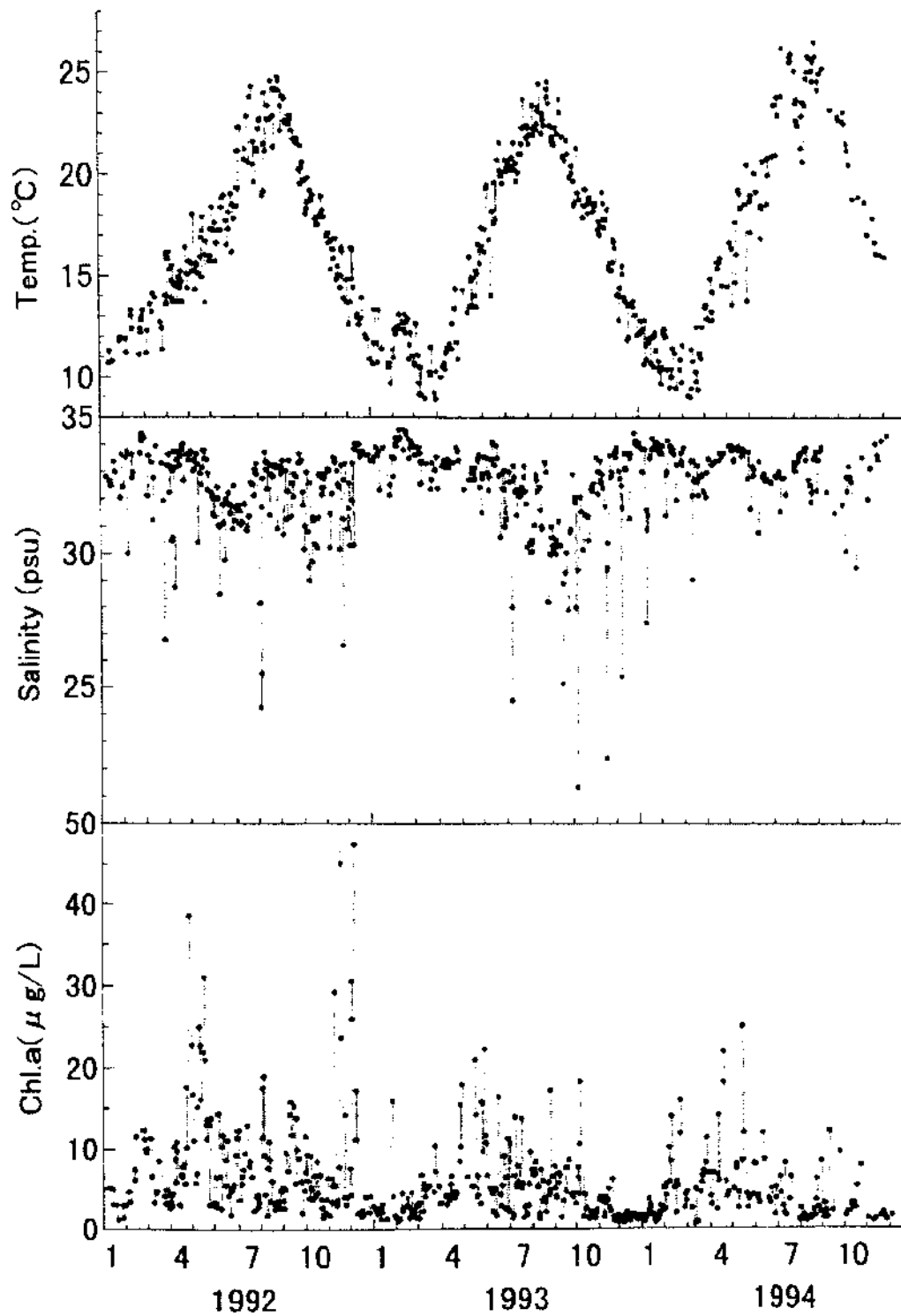
Figure 4. The temporal variation of temperature, salinity and chlorophyll a at the shoreline of the Hasaki Oceanographical Research Station.
