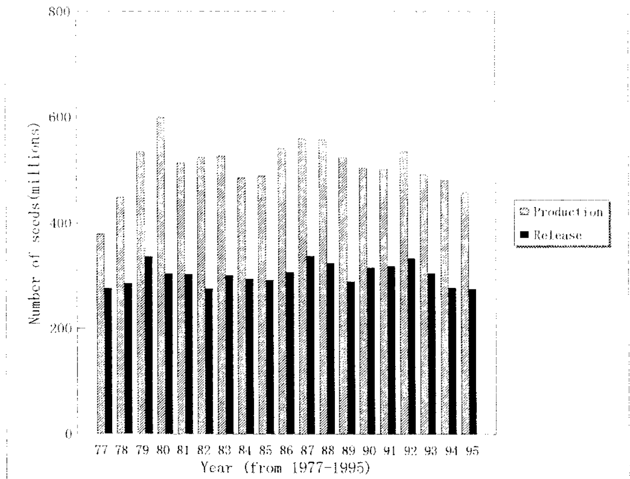
Figure 5. Statistics for artificial seed production and release of P. japonicus in Japan from 1977 to 1995 (courtesy of the Japan Sea-Farming Association).
