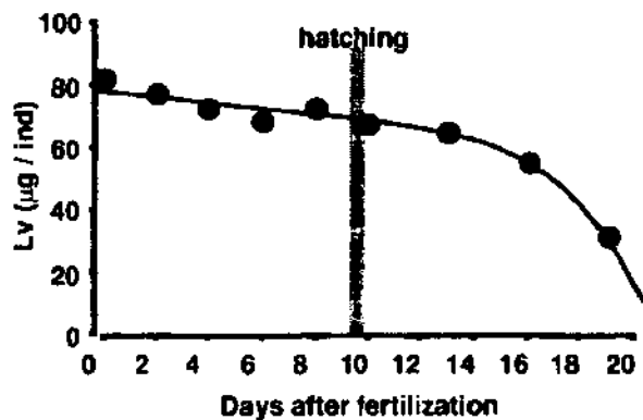
Figure 4. Changes in lipovitellin (Lv) content of developing eggs and larvae in barfin flounder. Hatching is represented by a vertical shaded bar.
