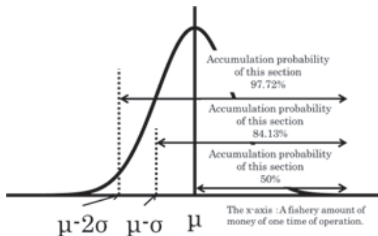
Fig. 56. Relations of the distribution of mean in the normal distribution and standard deviation and the data.
