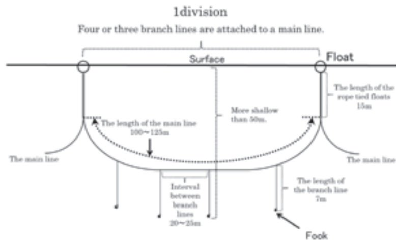
Fig. 46. Specifications of "Shallower set" fishing implements.
