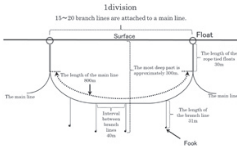
Fig. 47. Specifications of "Deeper set" fishing implements.
