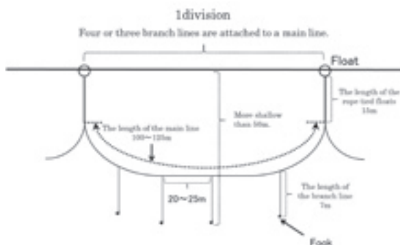
Fig. 39. Specifications of fishing implements.
