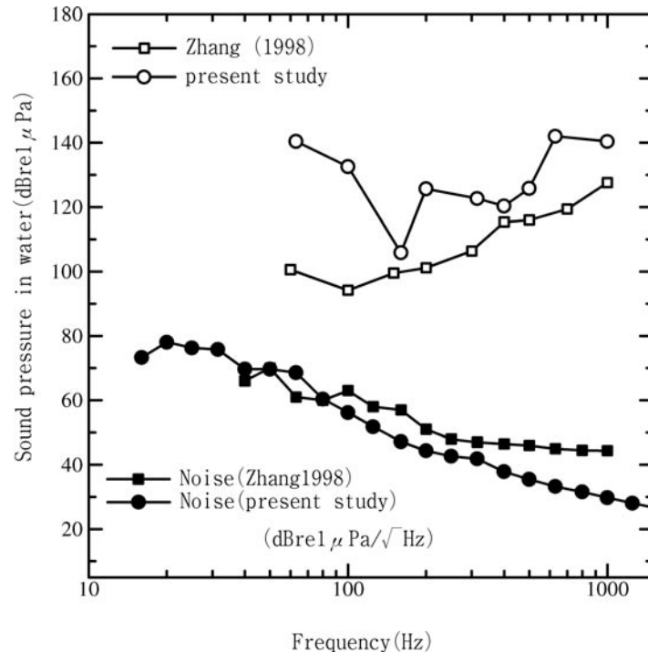
Fig. 1-12. Comparison of audiograms measured using two speakers facing each other to eliminate displacement (Zhang, 1998) and using sound stimulation in air (present study).
