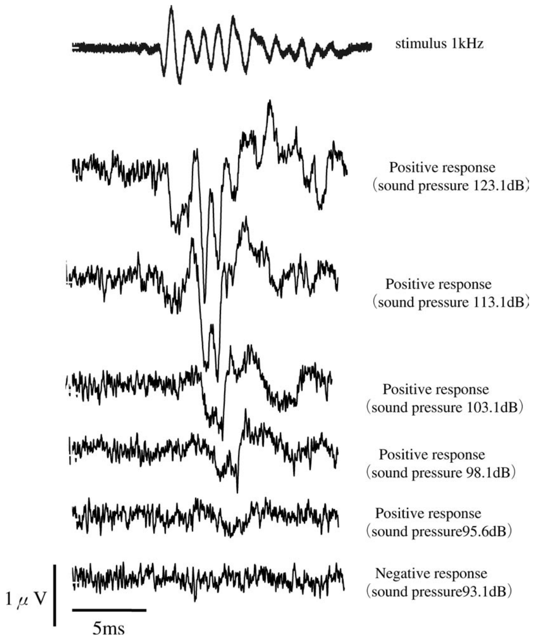
Fig. 3-6. The method to determine auditory thresholds.
