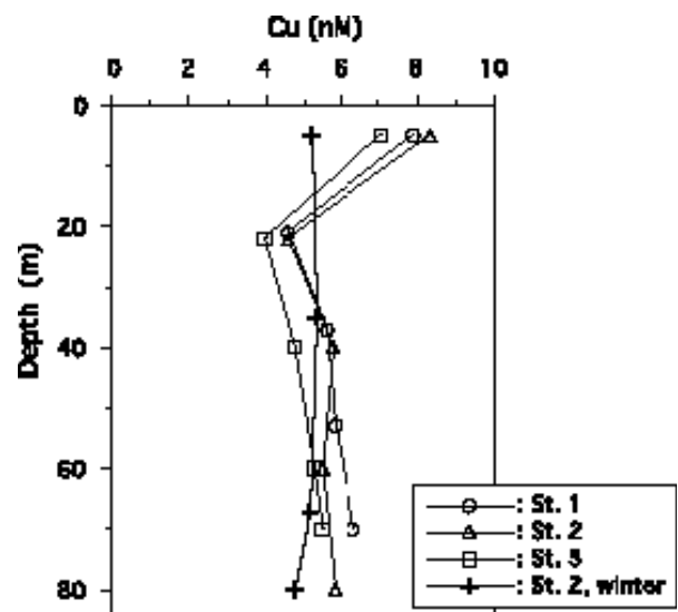
Fig. 5. Vertical profiles of Cu
