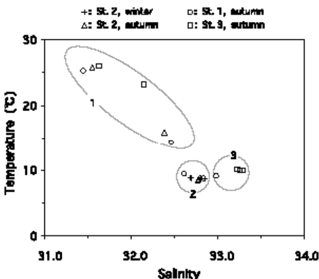
Fig. 4. T-S diagram. Three water masses were classified as "1", "2", and "3" corresponding to the water mass influenced by the discharge of the Huanghe and the Changjiang, the Yellow Sea cold bottom water (YSCBW), and the bottom water originated from the Kuroshio, respectively.
