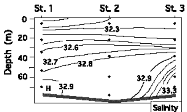
Fig. 3. Distributions of salinity
