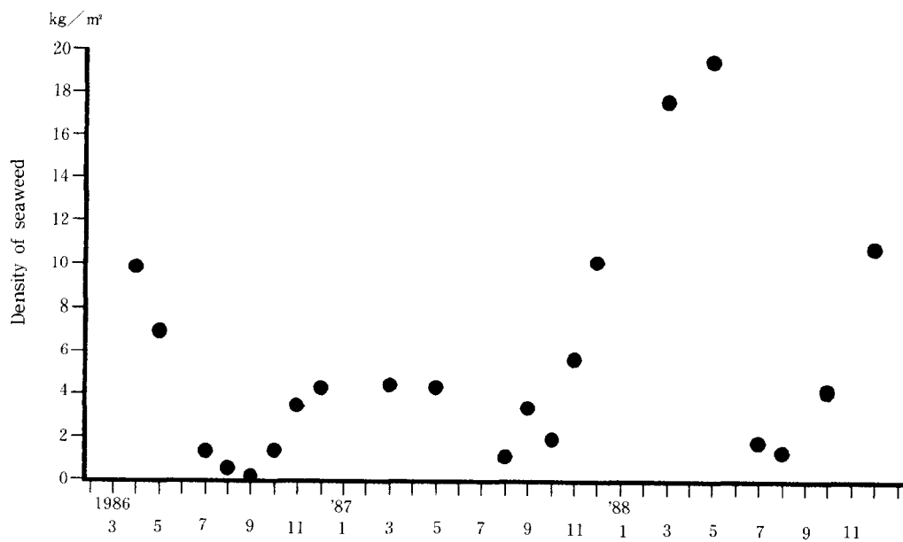
Fig. 2. Seasonal change of the density of seaweed (kg/m 2 ) in the man-made Sargassum forest.
