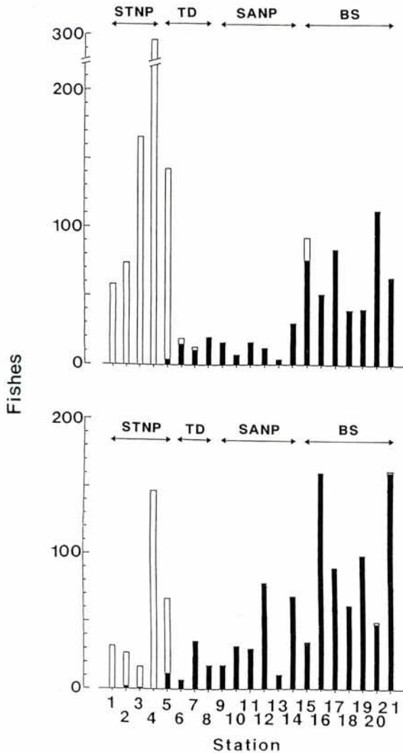
Fig. 7. Latitudinal changes in number of salmonids (closed histograms) and other epipelagic planktivorous fishes (open histograms) caught along a transect at 179° 30' W from mid-June to early July in 1992 (top) and 1993 (bottom). STNP: subtropical North Pacific, TD: Transition Domain, SANP: subarctic North Pacific, BS: Bering Sea.
