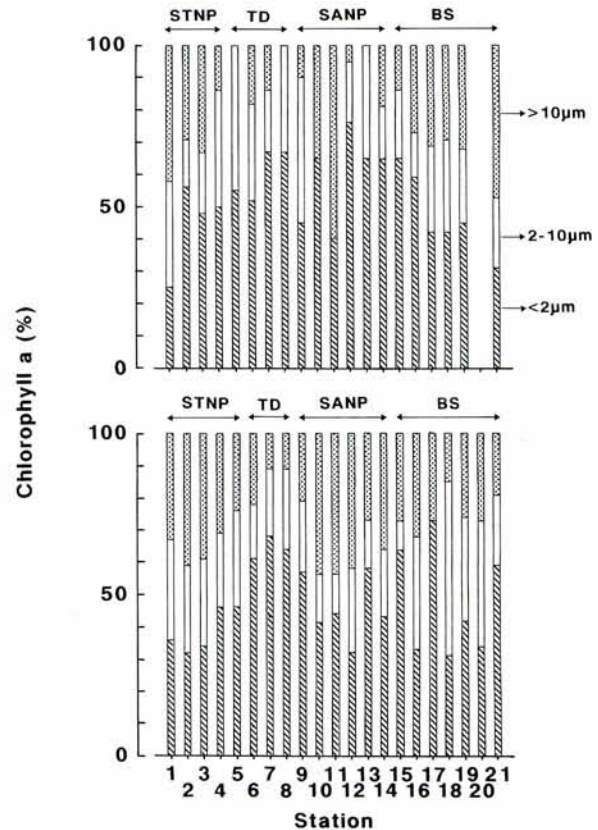
Fig. 4. Latitudinal changes in percentage of three size fractions of chlorophyll- a along a transect at 179° 30'W from mid-June to early July in 1992 (top) and 1993 (bottom). STNP: subtropical North Pacific, TD: Transition Domain, SANP: subarctic North Pacific, BS: Bering Sea.
