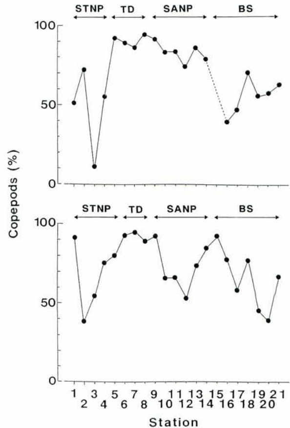
Fig. 6. Latitudinal changes in percentage of copepods in macrozooplankton biomass along a transect at 179^{\circ} 30'W from mid-June to early July in 1992 (top) and 1993 (bottom). STNP: subtropical North Pacific, TD: Transition Domain, SANP: subarctic North Pacific, BS: Bering Sea.
