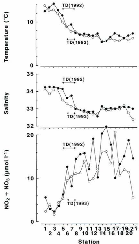
Fig. 2. Latitudinal changes in sea-surface temperature (top), sea-surface salinity (middle), and concentration of \text{NO}_2 + \text{NO}_3 (bottom) along a transect at 179° 30' W from mid-June to early July in 1992 (○) and 1993 (●). TD: Transition Domain.
