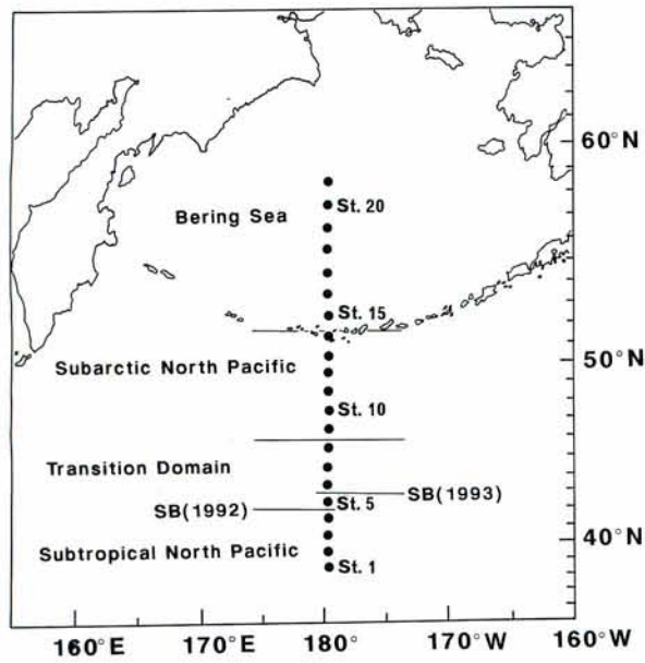
Fig. 1. Location of sampling stations during the cruises of the R/V Wakatake maru along a transect at 179° 30' W longitude from mid-June to early July in 1992 and 1993. The survey region was divided into four water masses: subtropical North Pacific, Transition Domain, subarctic North Pacific, and Bering Sea. SB: Subarctic Boundary.
