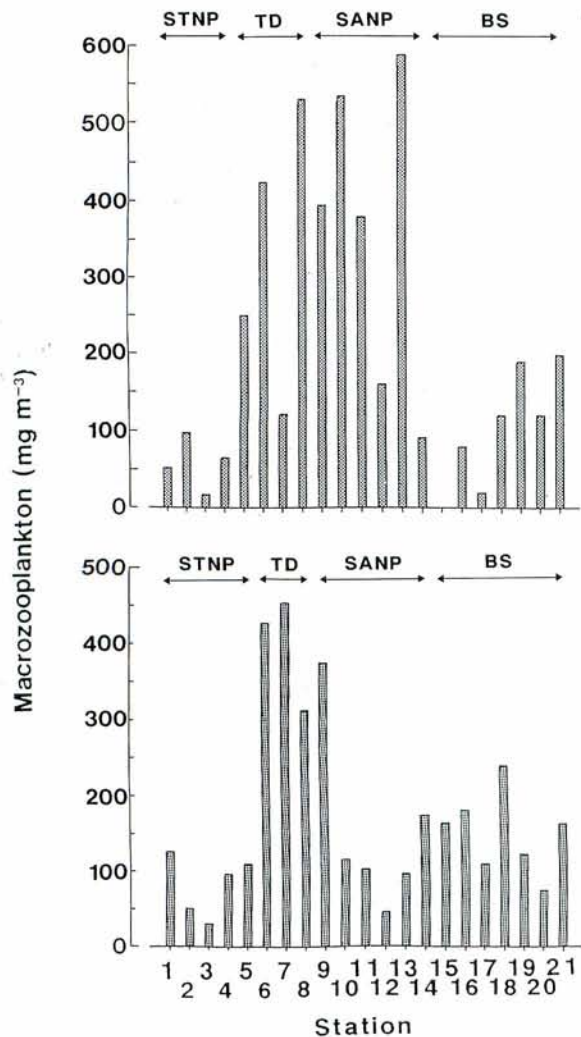
Fig. 5. Latitudinal changes in macrozooplankton biomass along a transect at 179^{\circ} 30'W from mid-June to early July in 1992 (top) and 1993 (bottom). STNP: subtropical North Pacific, TD: Transition Domain, SANP: subarctic North Pacific, BS: Bering Sea.
