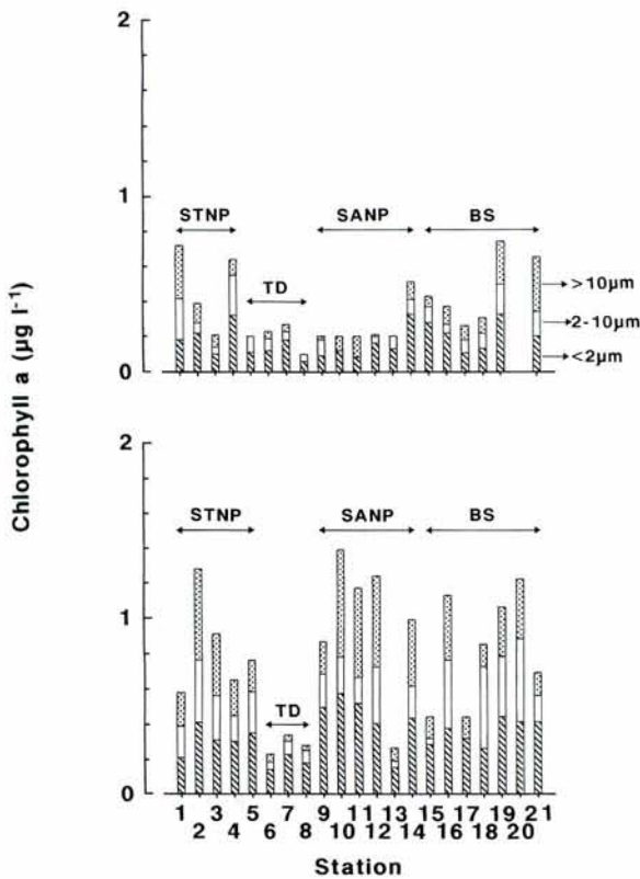
Fig. 3. Latitudinal changes in total chlorophyll- a concentration along a transect at 179° 30'W from mid-June to early July in 1992 (top) and 1993 (bottom). STNP: subtropical North Pacific, TD: Transition Domain, SANP: subarctic North Pacific, BS: Bering Sea.
