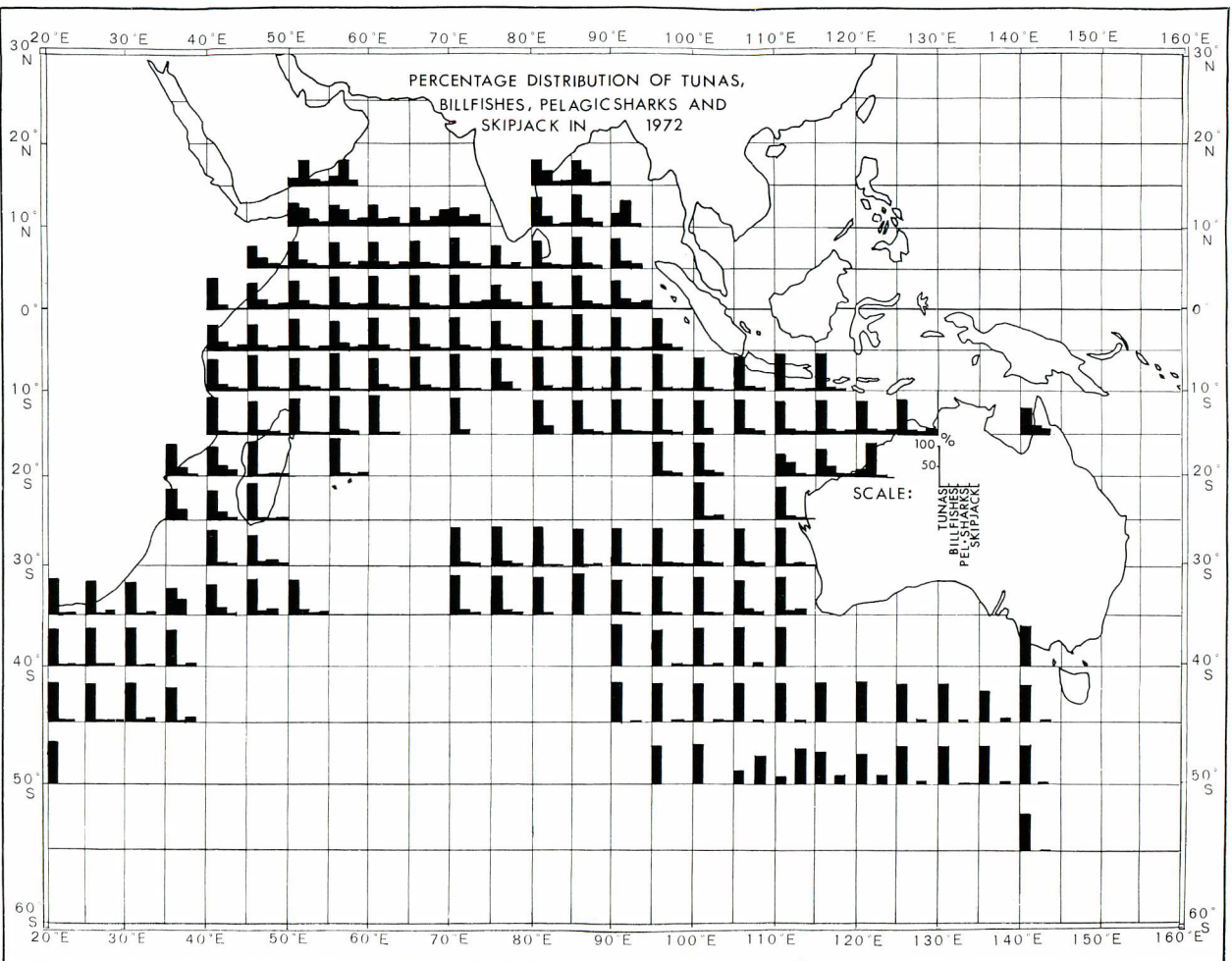
Fig. 2. Annual distribution of percentage composition of tunas, billfishes, pelagic sharks and skipjack in the Japanese tuna longline fishery, in the Indian Ocean, 1972.
