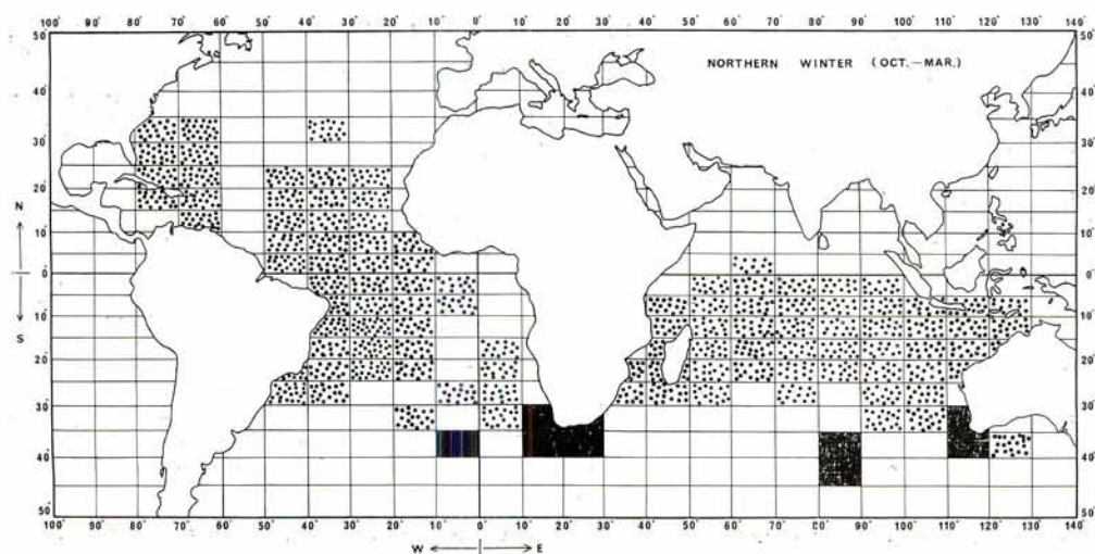
Fig. 3-2 Northern winter
