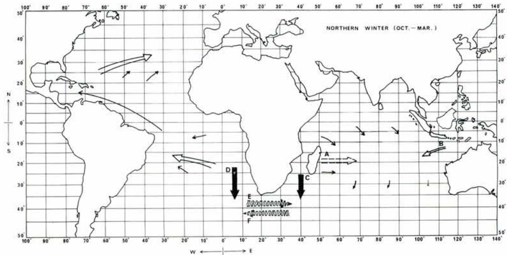
Fig. 4—2 Northern winter
