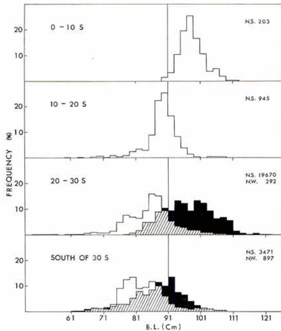
Fig. 5-1 Eastern areas of the South Atlantic Ocean (0°—20°E) Numerals denote number of measured fish
