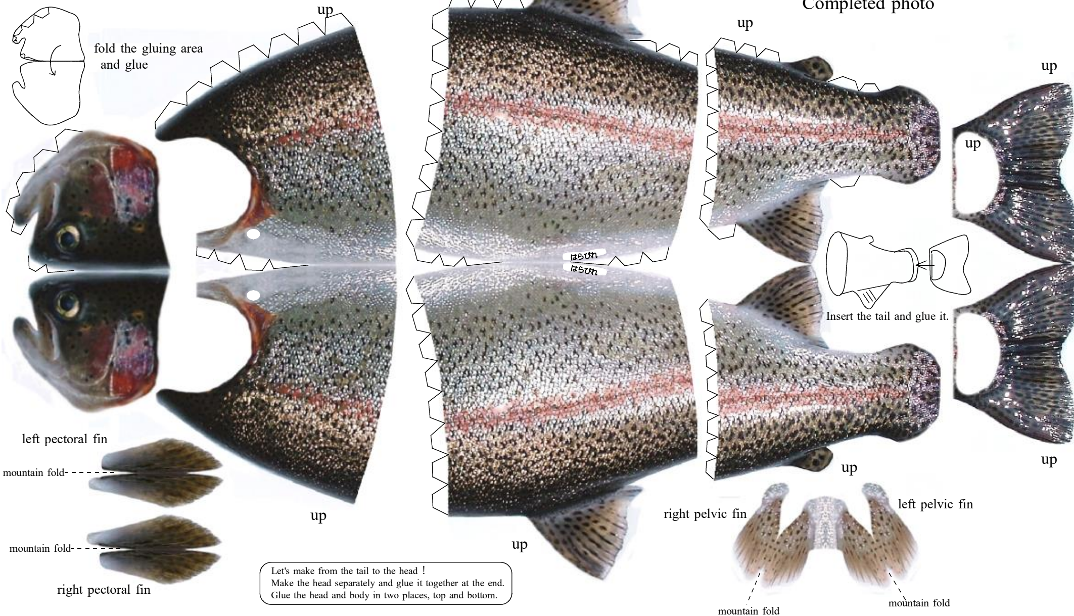
Completed photo
